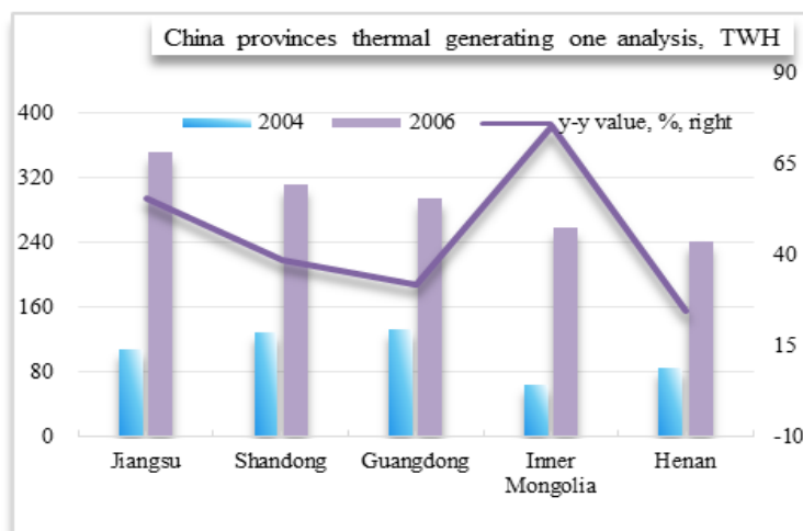
Figure 1 Thermal power generating status in provinces. [1]
